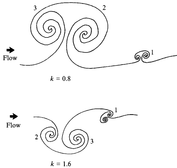
FIGURE 5. Schematic of observed vortex structure in the wake for indicated values of k . 1, shear-layer vortex; 2, dynamic stall vortex; 3, trailing-edge vortex.
