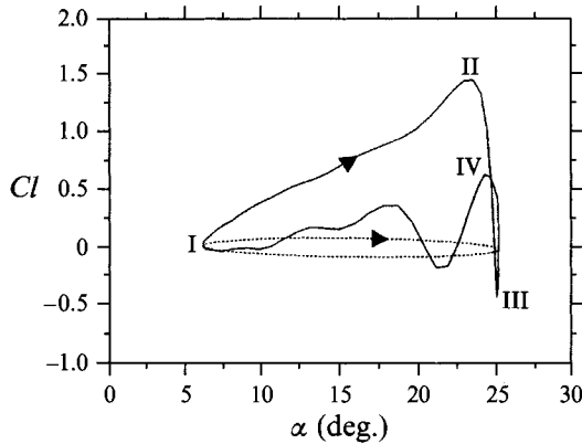
FIGURE 13. Estimated, unsteady component of Cl vs. \alpha obtained by adding the results of equation (1) (figure 12a) and the 'non-circulatory' component. The latter is represented by the dashed curve. k = 0.16 , R_c = 44000 , M = 0.019 .
