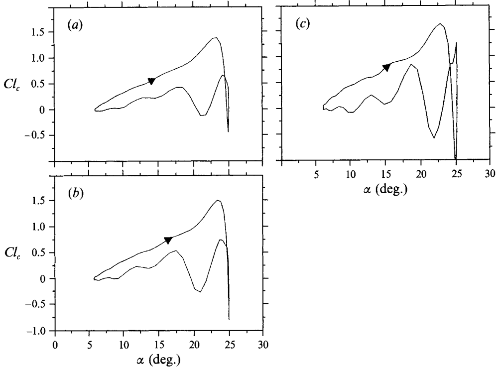
FIGURE 12. Estimated Cl_c vs. \alpha from the data of figure 9(b); \alpha = 15.3^\circ + 9.7^\circ \sin(2\pi ft - \frac{1}{2}\pi) , k = 0.16 . (a) to (c) obtained using equations (1) to (3) (see text), respectively.
