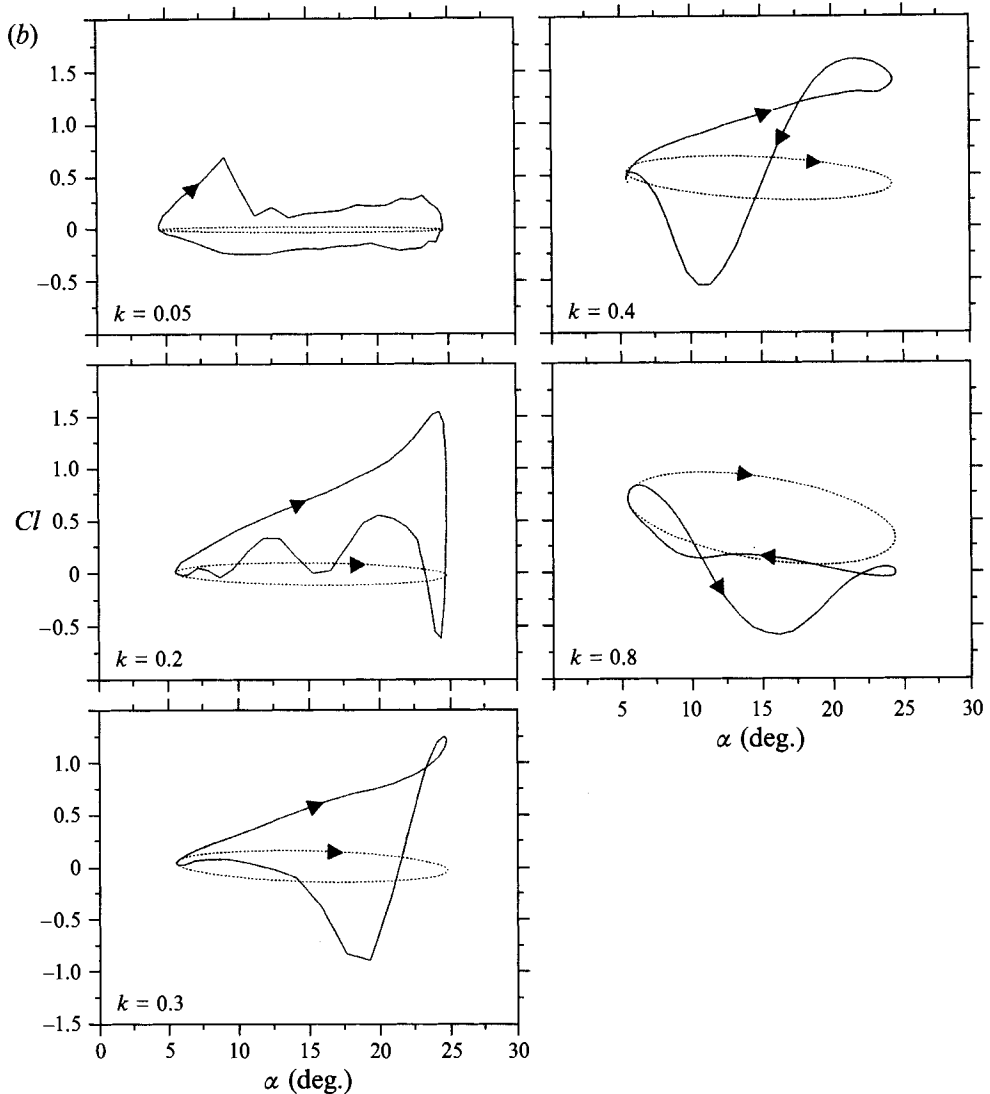
FIGURE 15. Effect of k for \alpha = 15.3^\circ + 9.7^\circ \sin(2\pi ft - \frac{1}{2}\pi) ; R_c = 44000 for k = 0.05 to 0.4 and R_c = 22000 for k = 0.8 . (a) \langle \omega_z \rangle c/U_\infty contours similar to the data of figure 9. (b) Estimated unsteady component of Cl vs. \alpha ; dashed curves represent non-circulatory component.
