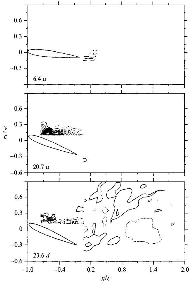
FIGURE 8. Contours of (\partial \langle u \rangle / \partial x + \partial \langle v \rangle / \partial y) , normalized by U_\infty / c , corresponding to the data of figure 7 for the indicated phases. Contour levels are same as in figure 7.
