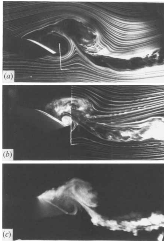
FIGURE 3. Flow-visualization photographs for the phase when the dynamic stall vortex and the trailing-edge vortex are shed into the wake ( \alpha \approx 25^\circ ); k = 0.2 , \alpha = 15^\circ + 10^\circ \sin 2\pi ft . (a) smoke wire placed upstream of airfoil leading edge, (b) smoke wire downstream of trailing edge, (c) smoke injection from a port on the airfoil lower surface.
