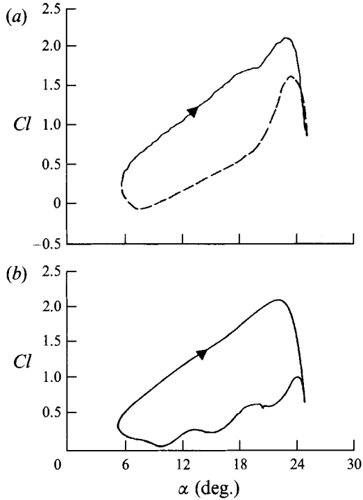
FIGURE 14. Total Cl variation with \alpha for k = 0.153 , \alpha = 15^\circ + 10^\circ \sin 2\pi ft : (a) experimental data of McAlister et al. (1982), R_c = 4.8 \times 10^5 , Mach number, M = 0.036 ; (b) computational data of L. N. Sankar (see Wu et al. 1990), R_c = 3.45 \times 10^6 , M = 0.283 .
