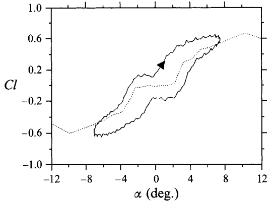
FIGURE 10. Cl vs. \alpha measured with a force balance for the case of figure 9(a): \alpha = 0^\circ + 7.2^\circ \sin 2\pi ft , k = 0.028 . —, Steady state variation of Cl with \alpha .
