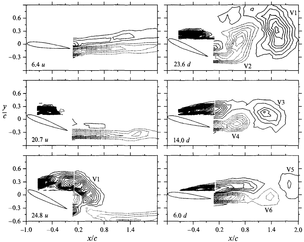
FIGURE 7. Contours of spanwise vorticity \omega_z , normalized by U_\infty/c , for indicated \alpha ; k = 0.2 , R_c = 44000 , \alpha = 15^\circ + 10^\circ \sin 2\pi ft . Contour levels for —, positive vorticity start at 0.5 and ---, for negative vorticity at -0.5 and are at an interval of 0.5.
