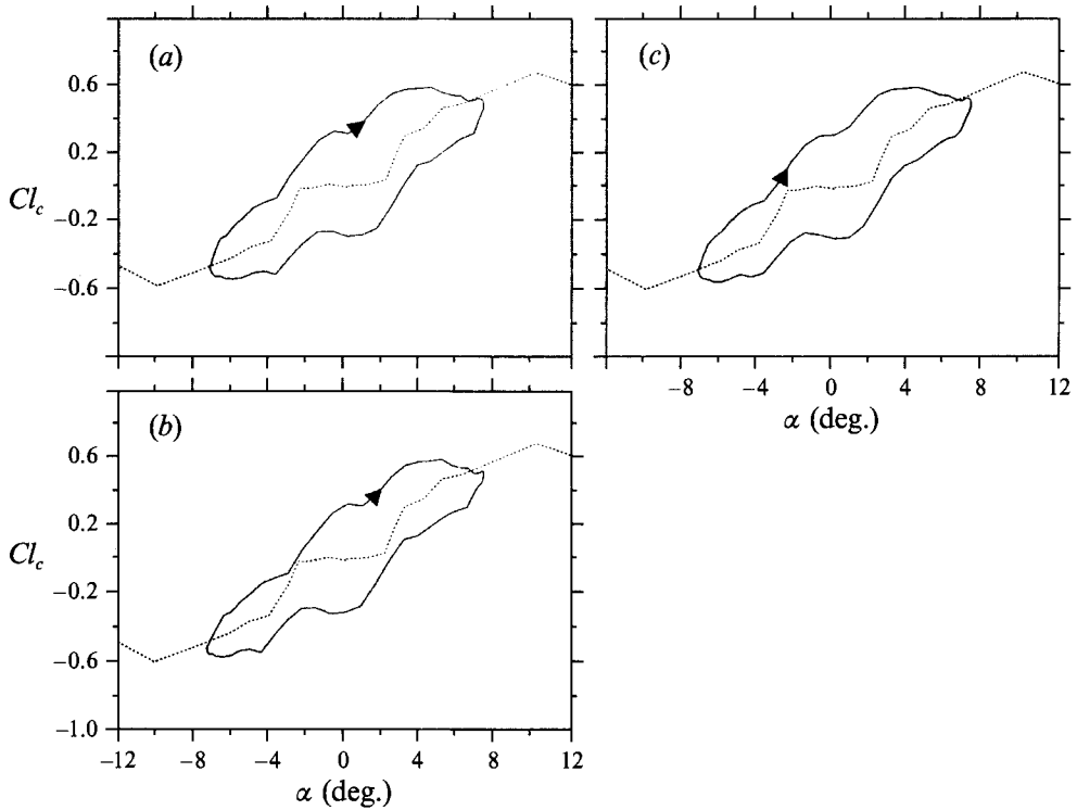
FIGURE 11. Estimated Cl_c vs. \alpha from the data of figure 9(a); \alpha = 0^\circ + 7.2^\circ \sin 2\pi ft , k = 0.028 . (a) to (c) obtained using equations (1) to (3) (see text), respectively.
