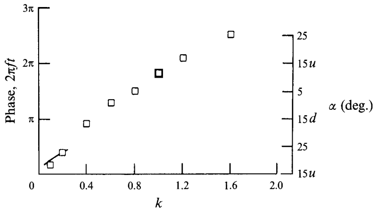
FIGURE 6. Approximate phase, when the centre of the DSV is above the trailing edge, at different k . —, data of McAlister et al. (1978).
