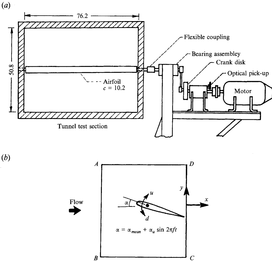
FIGURE 1. (a) Schematic of wind-tunnel test section and airfoil oscillation mechanism. (b) Coordinate system and control volume for calculation of unsteady circulation.
