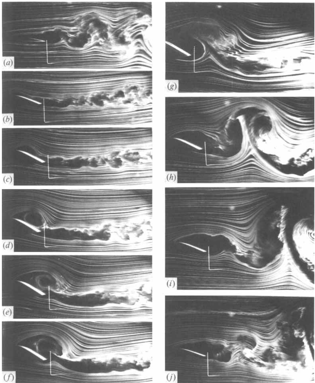
FIGURE 2. Smoke-wire flow-visualization photographs at different phases of the oscillation cycle; k = 0.2 , \alpha = 15^\circ + 10^\circ \sin 2\pi ft . Approximate \alpha for (a)–(j) are 5^\circ u , 14^\circ u , 20^\circ u , 22^\circ u , 24^\circ u , 25^\circ u , 25^\circ d , 20^\circ d , 16^\circ d , 12^\circ d , respectively; u and d denote increasing and decreasing \alpha .
