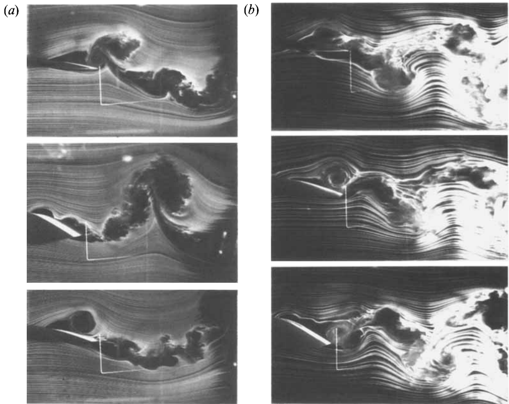
FIGURE 4. Smoke-wire flow visualization for two different k ; R_e = 22000 , \alpha = 15^\circ + 10^\circ \sin 2\pi ft . (a) k = 0.8 ; (b) k = 1.6 . Approximate \alpha from top to bottom for (a): 7^\circ u , 23^\circ u , 13.5^\circ d and for (b): 5^\circ , 15.5^\circ u , and 25^\circ .
