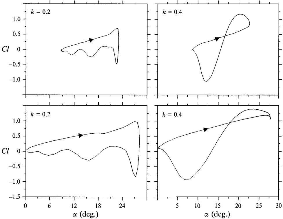
FIGURE 16. Estimated Cl vs. \alpha for two different amplitudes of oscillation for indicated values of k . Top row: \alpha = 15.7^\circ + 7.2^\circ \sin(2\pi ft - \frac{1}{2}\pi) ; Bottom row: \alpha = 14.1^\circ + 14.1^\circ \sin(2\pi ft - \frac{1}{2}\pi) .
