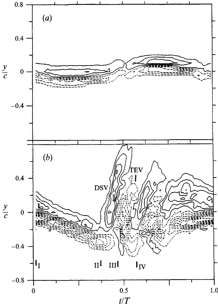
FIGURE 9. Temporal distributions of \langle \omega_z \rangle c / U_\infty over a cycle, measured at x/c = 0.3 ; R_c = 44000 . Contour levels for —, positive vorticity start at 0.5 and ---, for negative vorticity start at -0.5 and are at an interval of 0.5. (a) \alpha = 0^\circ + 7.2^\circ \sin 2\pi ft , k = 0.028 , (b) \alpha = 15.3^\circ + 9.7^\circ \sin(2\pi ft - \frac{1}{2}\pi) , k = 0.16 .
